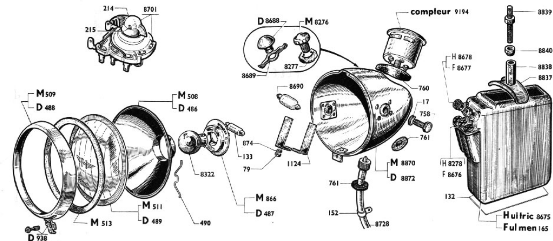
Phare complet Marchal 8869
