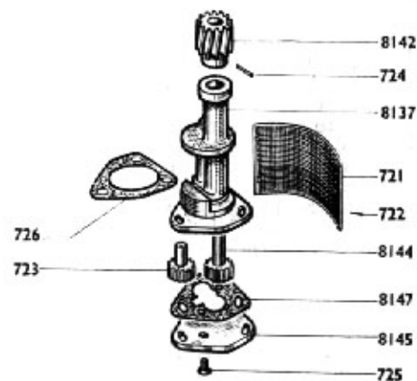
Pompe complete 8136
