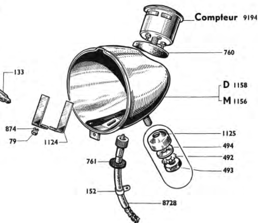
Phare complet Marchal 1155
