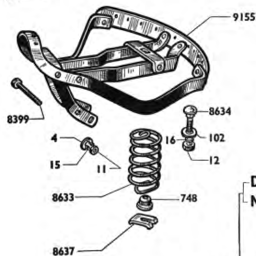
Phare complet Ducellier 1157
